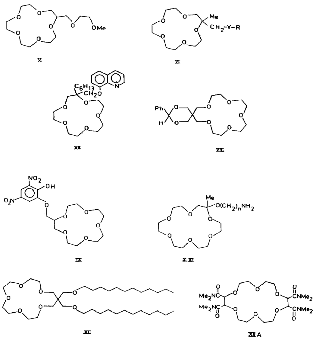
Fig. 25. Category 2 crown-related macrocycles (carrying electrically neutral substituents on the crown ring): V–XII A (for VI, Y can be O, S or NH and R can be a long group; X, n = 5 ; XI, n = 2 ).
