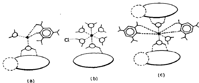
Fig. 18. A schematic view of products wherein the M^{z+} -crown interaction is missing: (a) [\text{Li}(\text{pic})(\text{H}_2\text{O})_2]\text{B15C5} ; (b) [\text{Mg}(\text{H}_2\text{O})_6](12\text{C4})\text{Cl}_2 ; (c) [\text{Ca}(\text{pic})_2(\text{H}_2\text{O})_3]\text{B15C5} .
