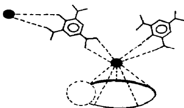
Fig. 13. A schematic view of a large-cation anion-paired encapsulate, viz. \text{Cs(pic)(B15C5)} .
