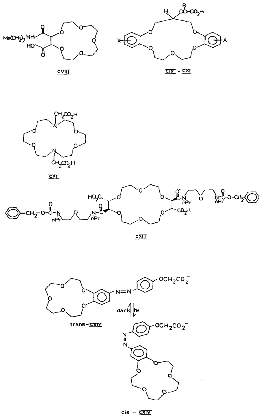
Fig. 47. Category 7 crown-related macrocycles (anionic macrocycles) CVIII-CXIX : CIX , \text{R} = \text{X} = \text{H} ; CX , \text{R} = (\text{CH}_2)_7\text{Me} , \text{X} = \text{H} ; CXI , \text{R} = \text{H} , \text{X} = \text{C}(\text{Me})_3 ; CXVIII , \text{R} = \text{NO}_2 ; CXIX , \text{R} = \text{CF}_3 .
