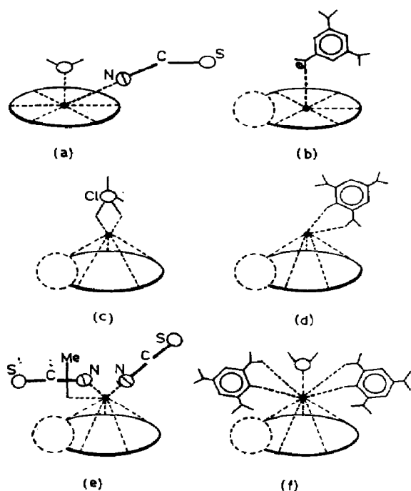
Fig. 11. A schematic view of selected cation-cavity comparable anion-paired encapsulates: (a) [\text{NaNCS}(\text{15C5})(\text{H}_2\text{O})] moiety of \text{NaNCS}(\text{15C5}) \cdot \frac{1}{2}\text{H}_2\text{O} ; (b) \text{Na}(\text{dnb})(\text{B15C5}) \cdot \text{H}_2\text{O} ; (c) \text{NaClO}_4(\text{B15C5}) ; (d) \text{Na}(\text{pic})(\text{B15C5}) ; (e) \text{Ca}(\text{NCS})_2(\text{B15C5}) \cdot \text{MeOH} ; (f) \text{Ba}(\text{pic})_2(\text{B15C5}) \cdot \text{H}_2\text{O} .
