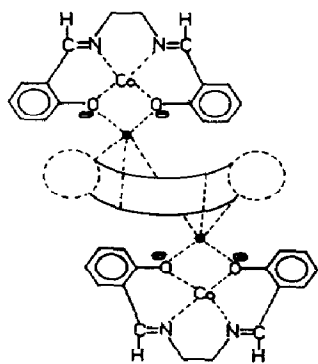
Fig. 15. A schematic view of "bimetallic" (\text{Co}(\text{salen})\text{Na})_2(\text{DC18C6 } \textit{cis-anti-cis}) .
