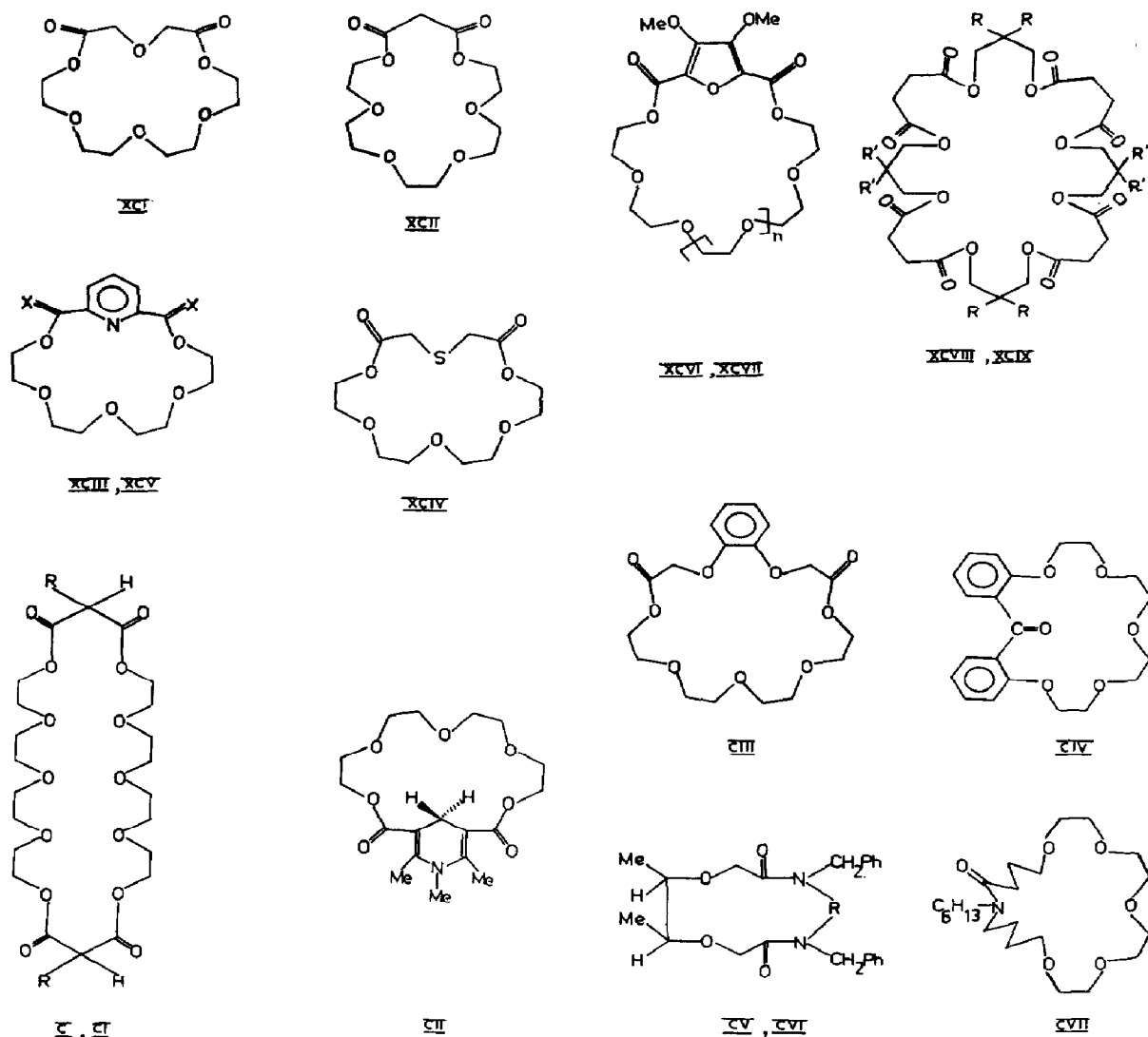
Fig. 45. Category 6 crown-related macrocycles (carrying oxo- and amide-substituents with or without heterocyclic nuclei) XCI – CVII : XCIII , X = O; XCIV , X = S; XCVI , n = 1 ; XCVII , n = 2 ; XCVIII , R = H, R' = Me; XCIX , R = R' = Me; C , R = n -C 8 H 17 ; CI , R = n -C 12 H 25 ; CV , R = CH 2 (CH 2 OCH 2 ) 3 CH 2 ; CVI , R = (CH 2 ) 12 .
